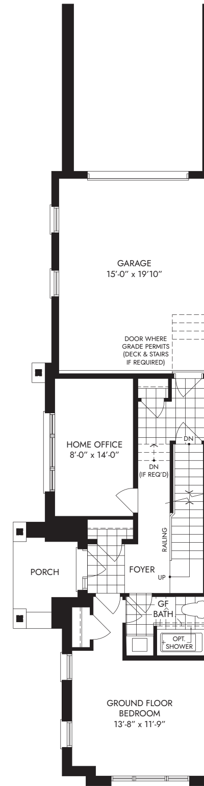
GROUND FLOOR ELEV. C
