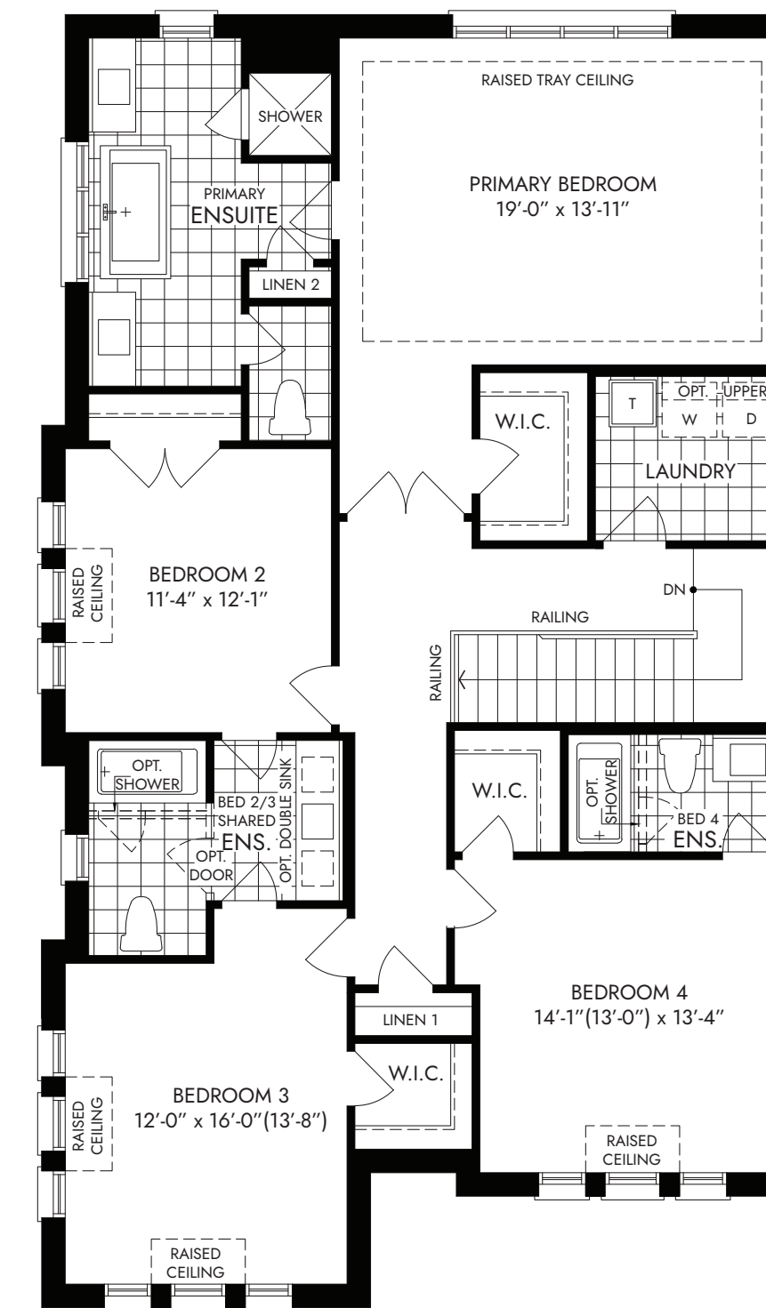
SECOND FLOOR (ELEV. A) - 4 BED
