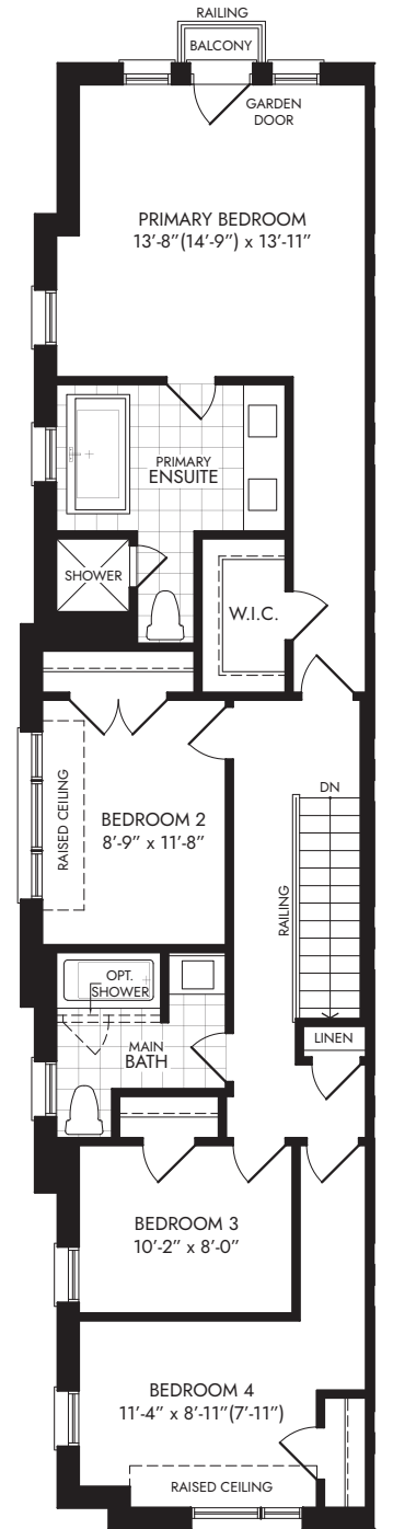
UPPER FLOOR ELEV. C
