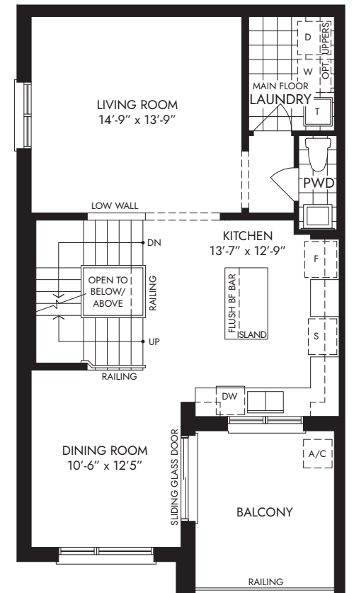
MAIN FLOOR ELEV. C
