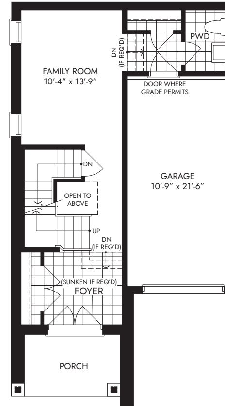
GROUND FLOOR ELEV. C
